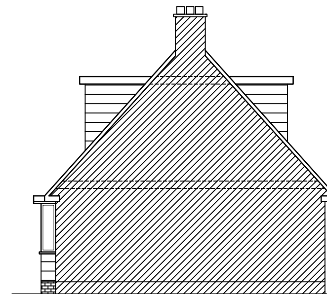
SIDE ELEVATION EXISTING (PARTY WALL SIDE)
