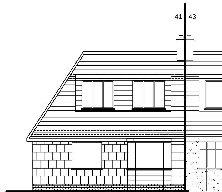
FRONT ELEVATION EXISTING
