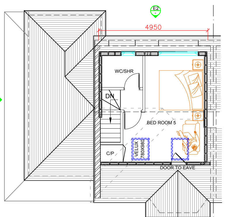
PROPOSED LOFT PLAN SCALE= 1:100
