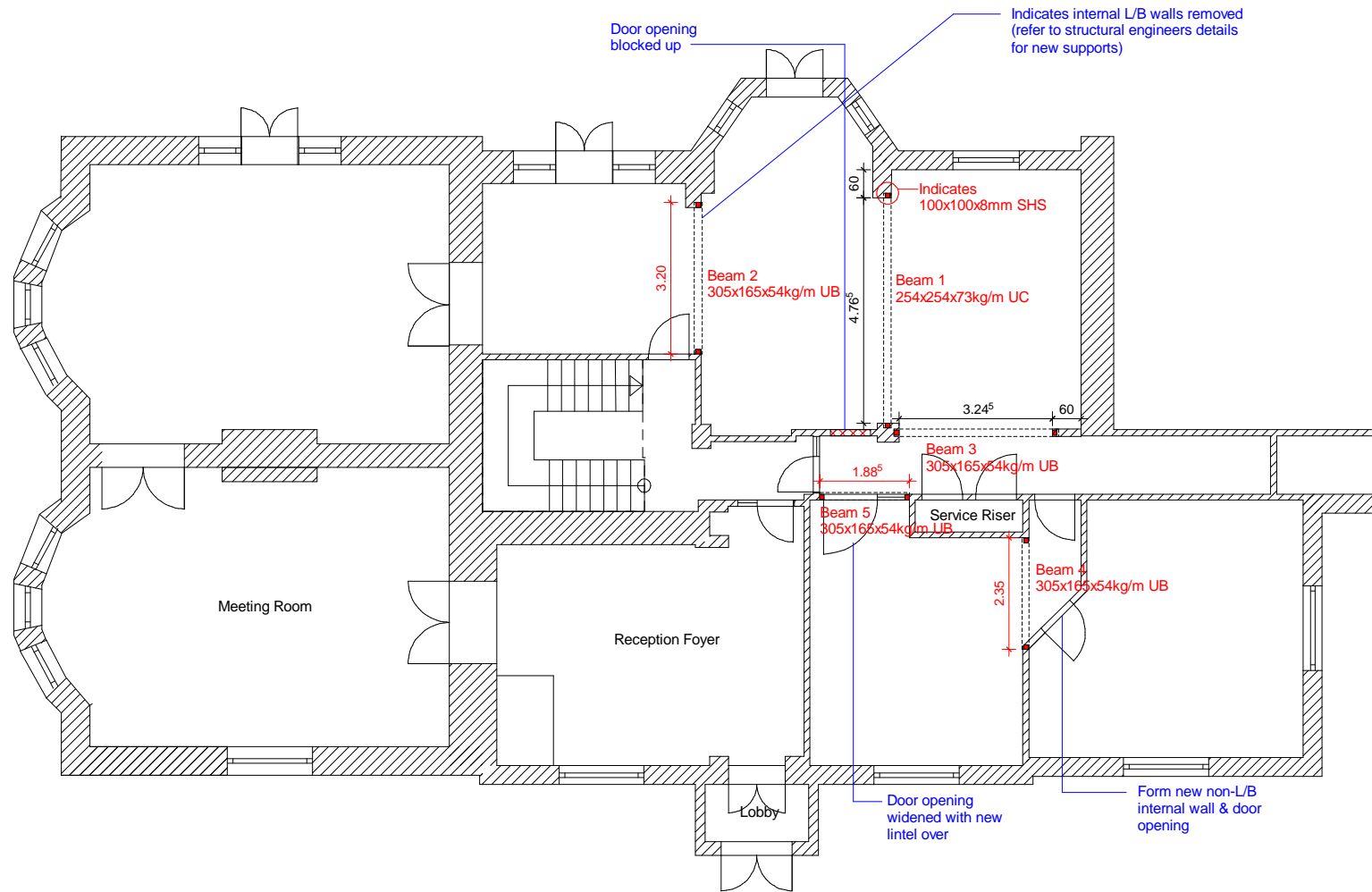
PROPOSED GROUND FLOOR LAYOUT - STRUCTURAL ALTERATIONS
