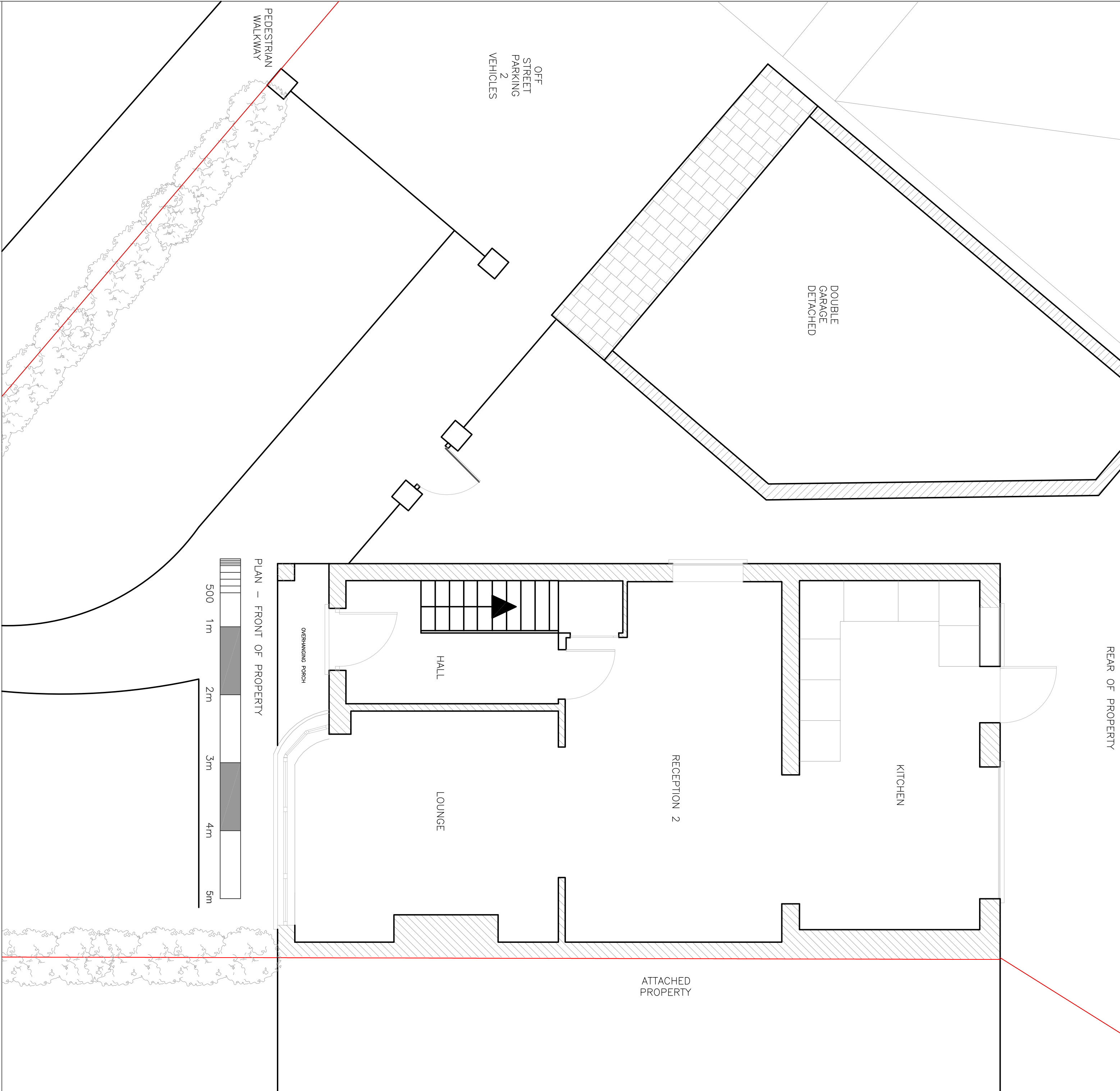
A 229 Existing Plan View Ground Floor Scale: 1:50 at A1
