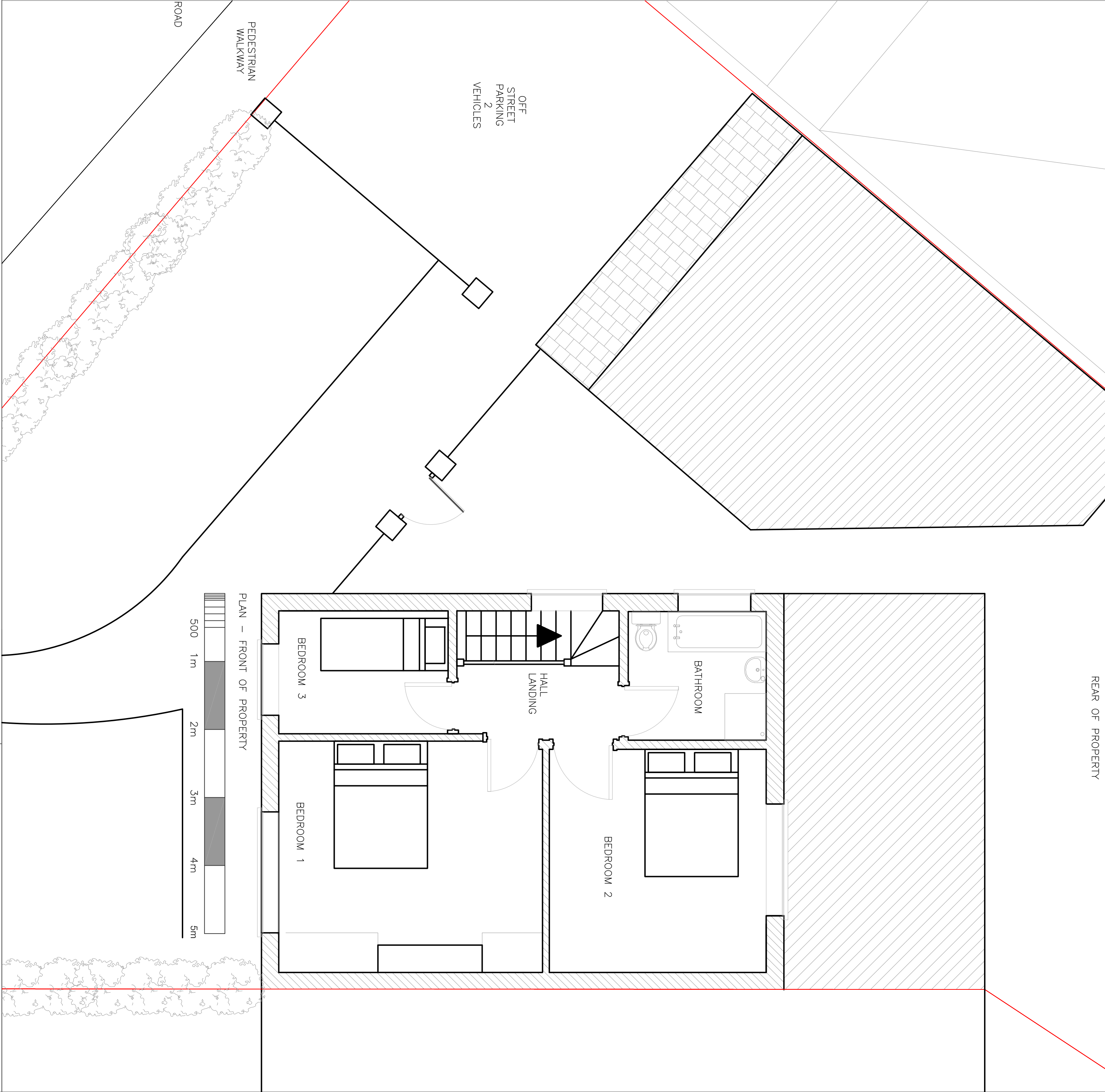
A 230 Existing Plan View First Floor Scale: 1:50 at A1
