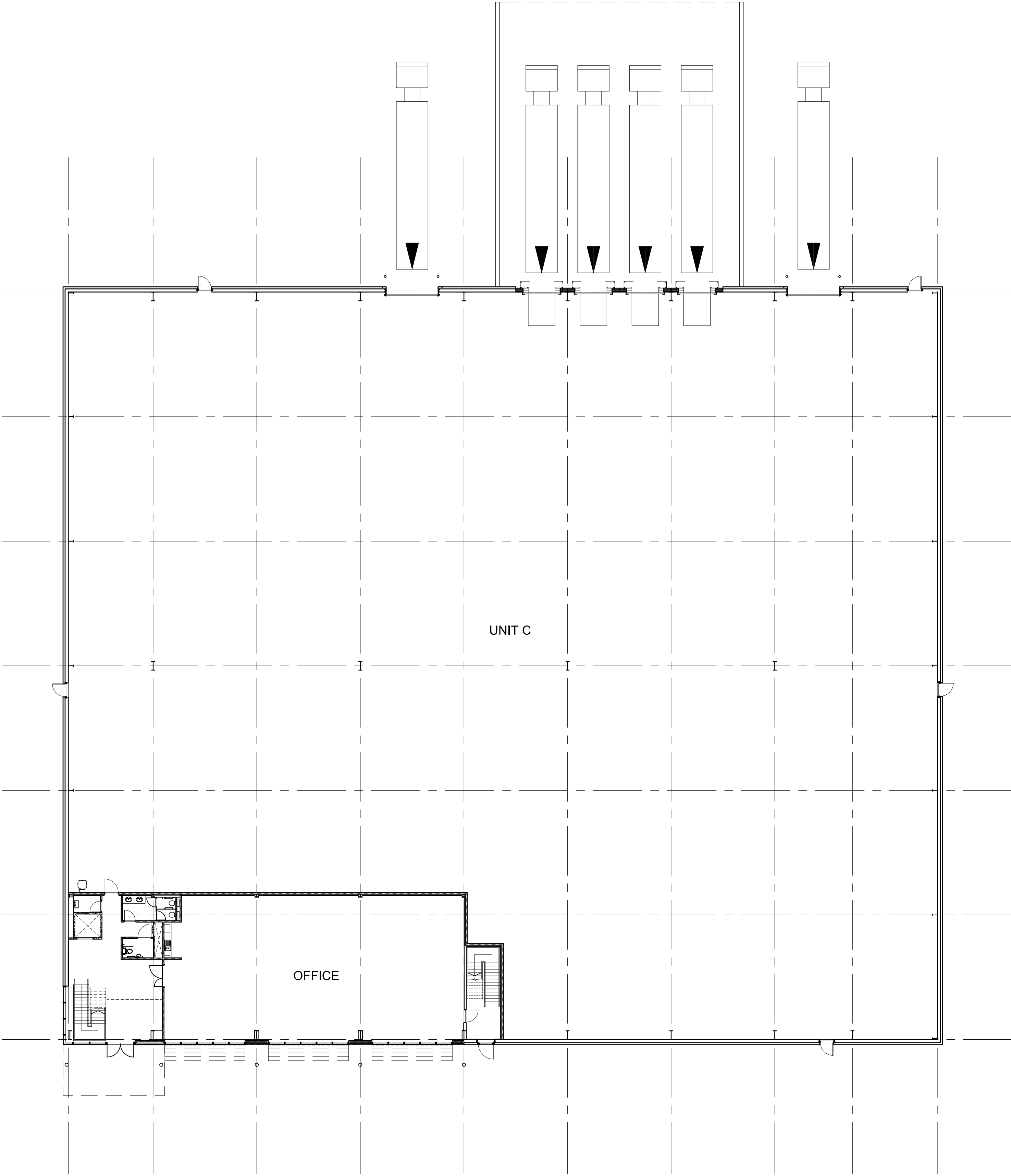
01 UNIT C - GROUND FLOOR PLAN 102 1:200
