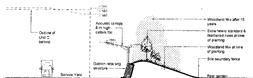
02 SECTION A-A 10 (Landscape Information from BCA drawing DMC) 1:200
