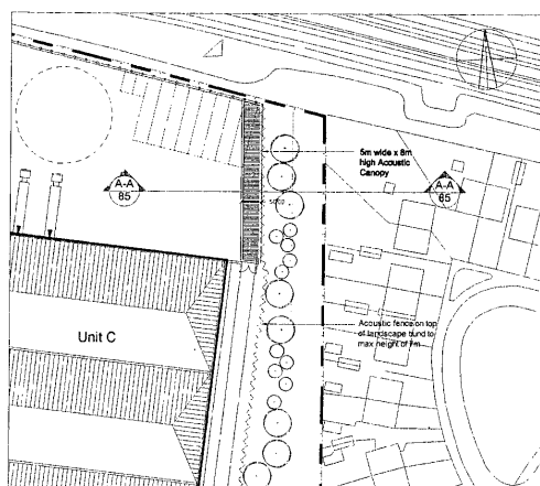
01 UNIT C PLAN 85 1-500
