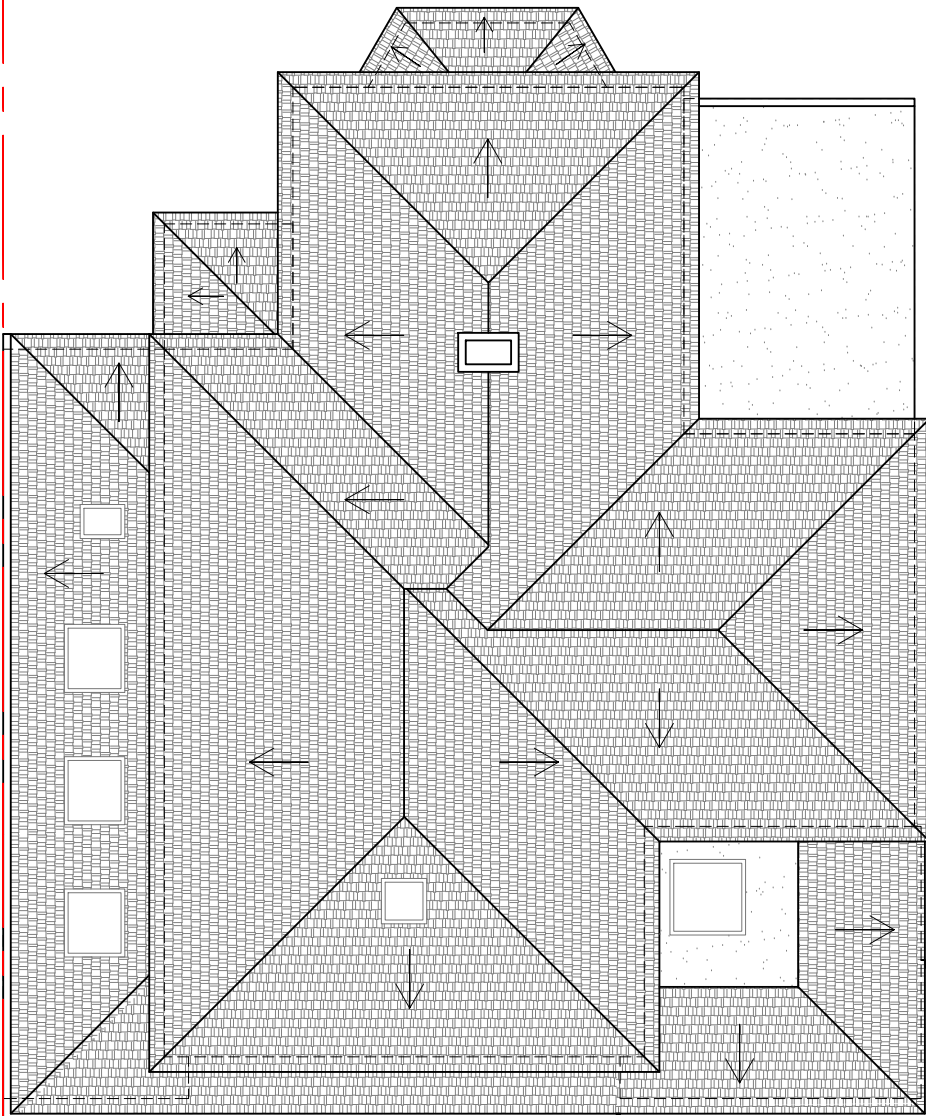
ROOF PLAN-PROPOSED
