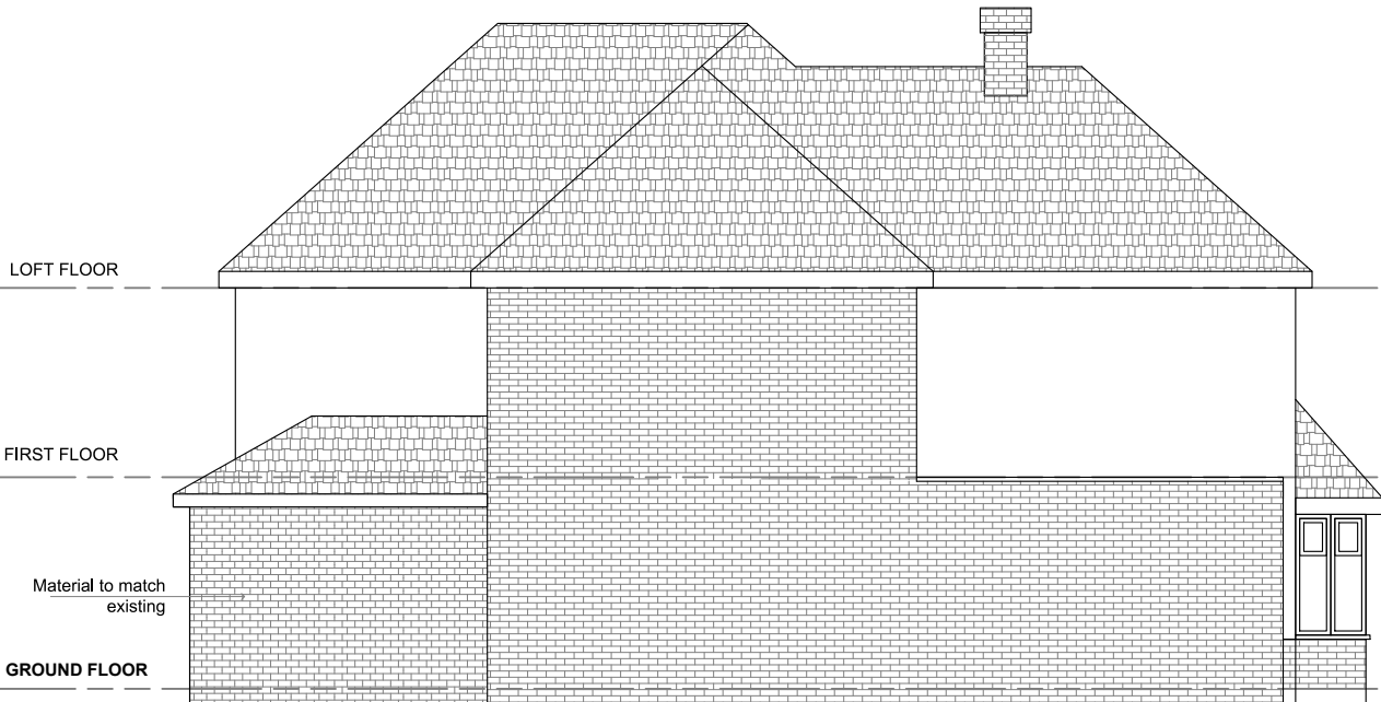
LEFT HAND SIDE ELEVATION-PROPOSED
