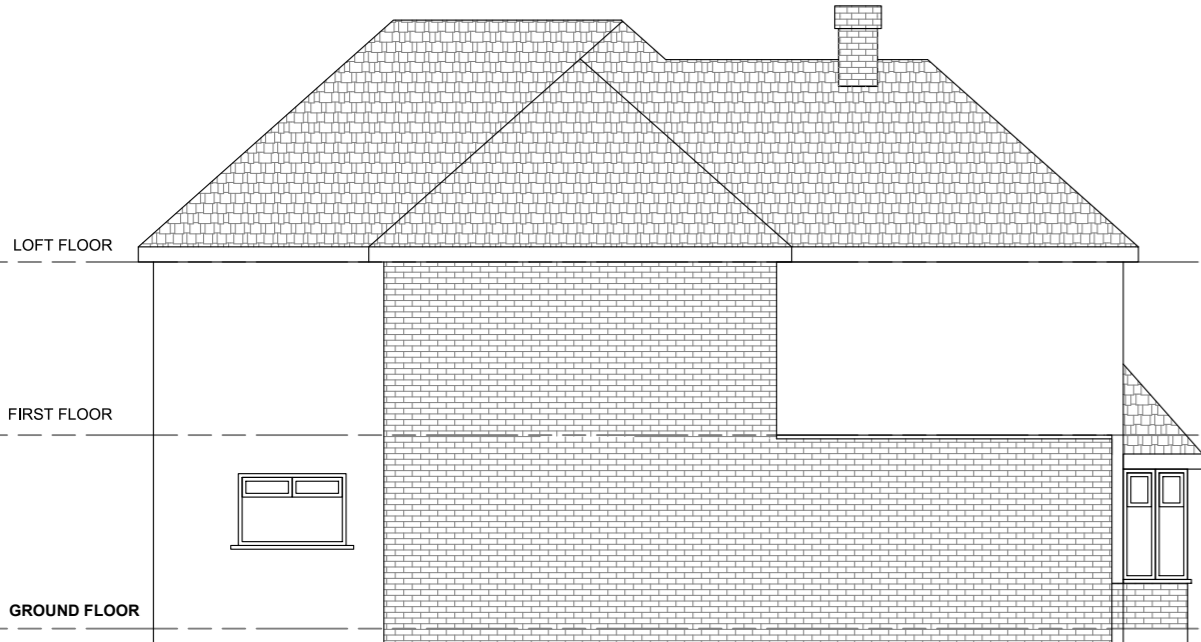
LEFT HAND SIDE ELEVATION-EXISTING
