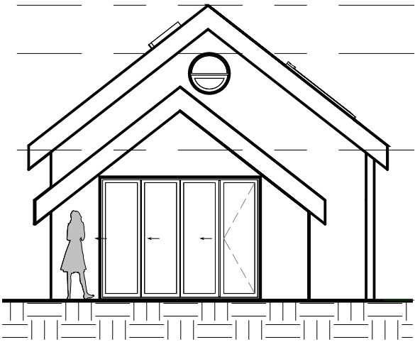
North Elevation 1 : 100
