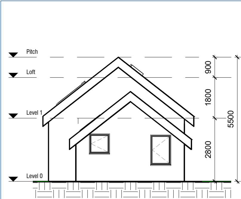
South Elevation 1 : 100
