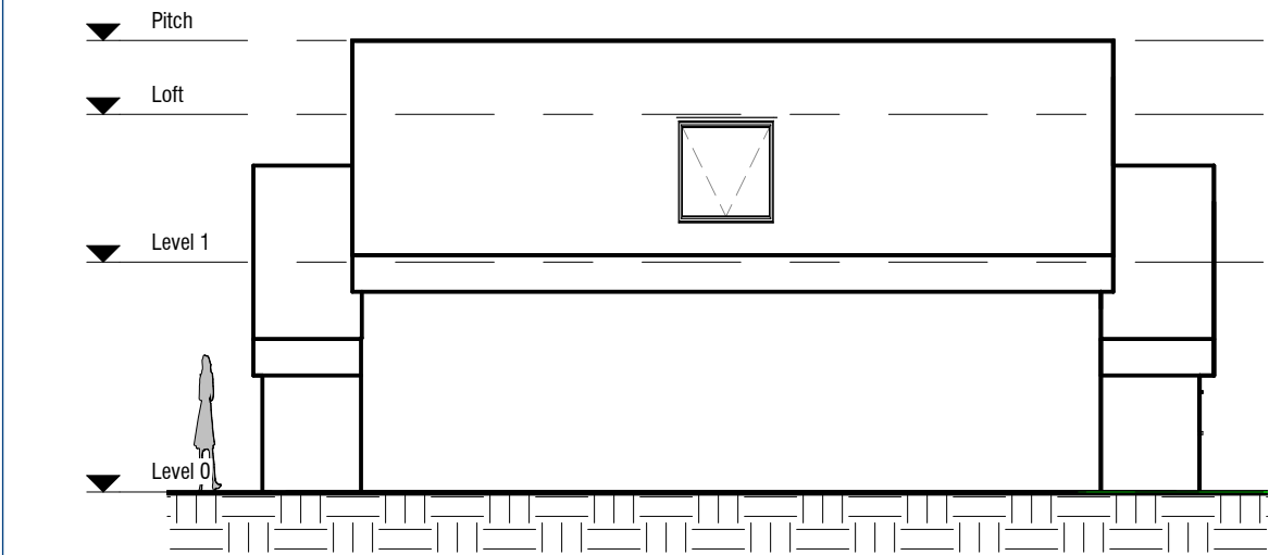
West Elevation 1 : 100
