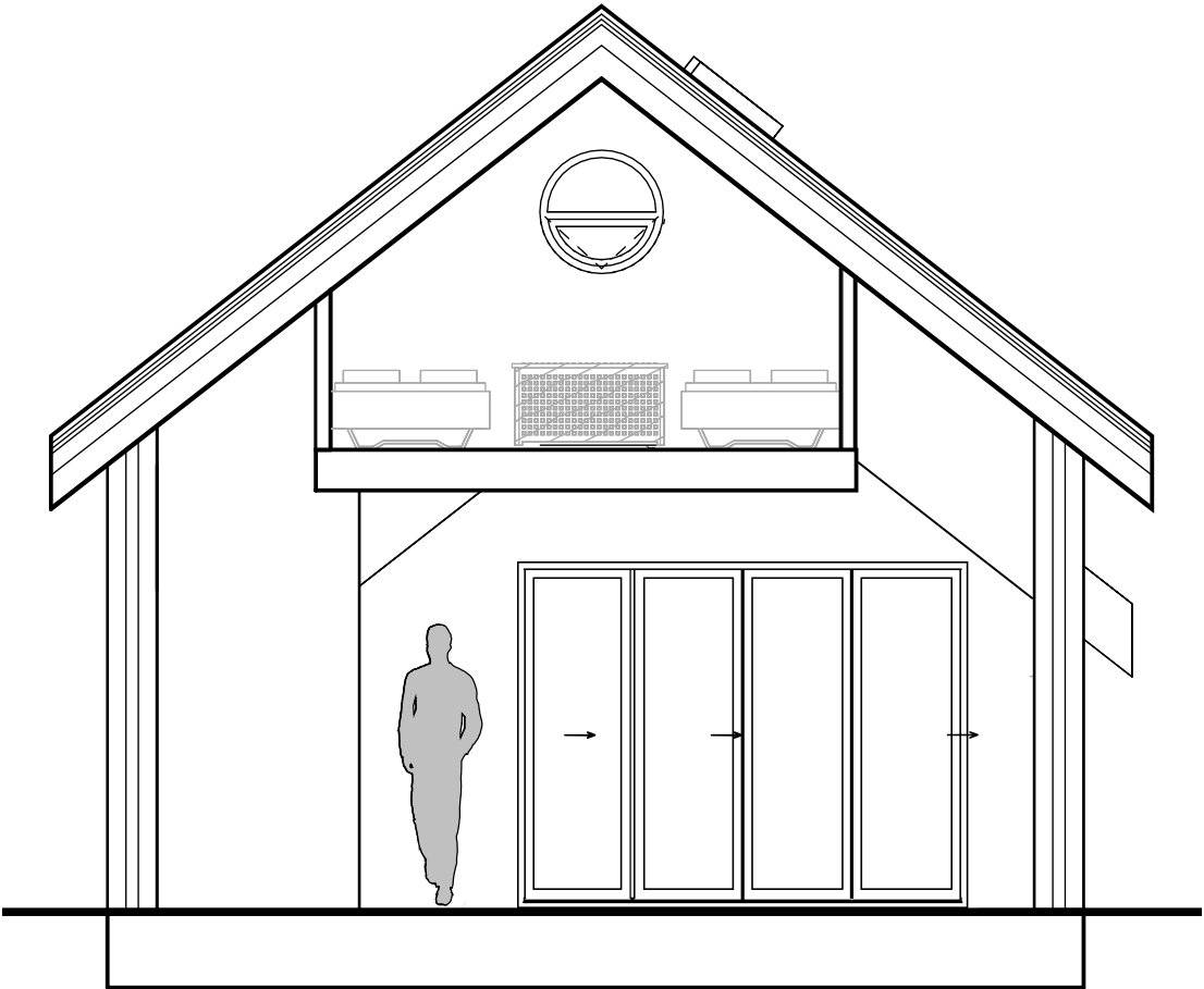
Section East-West 1 : 50
