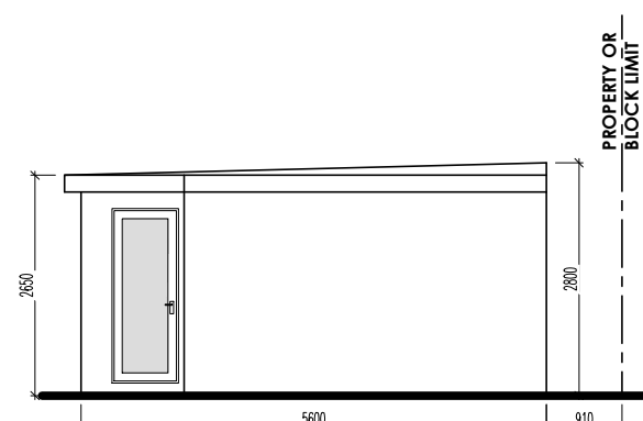
PROPOSED SIDE ELEVATION (FROM NO.83) SCALE 1/100
