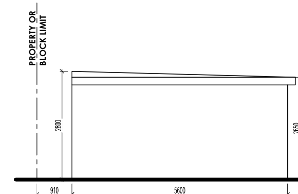
PROPOSED SIDE ELEVATION (FROM NO.79) SCALE 1/100
