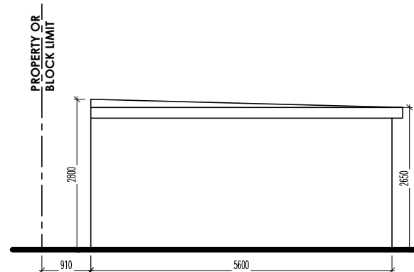
EXISTING SIDE ELEVATION (FROM NO.79) SCALE 1/100
