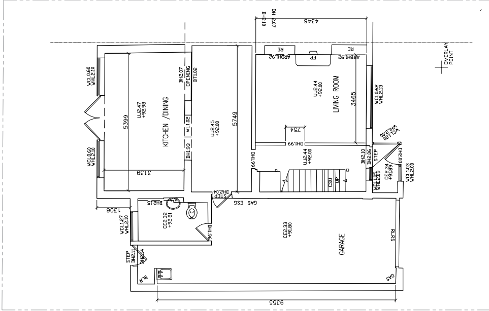
01 EXISTING GROUND FLOOR
