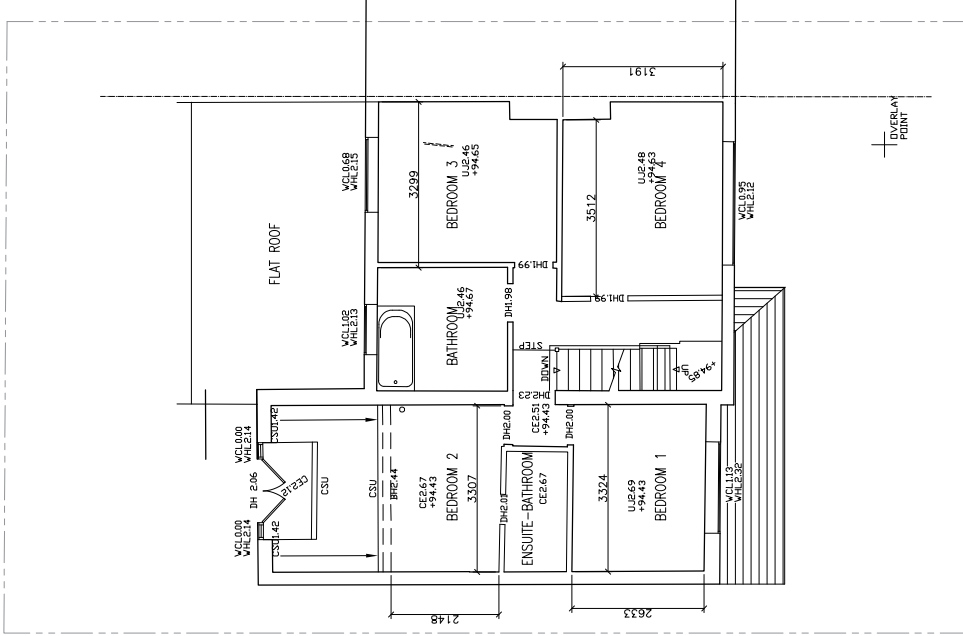
02 EXISTING FIRST FLOOR
