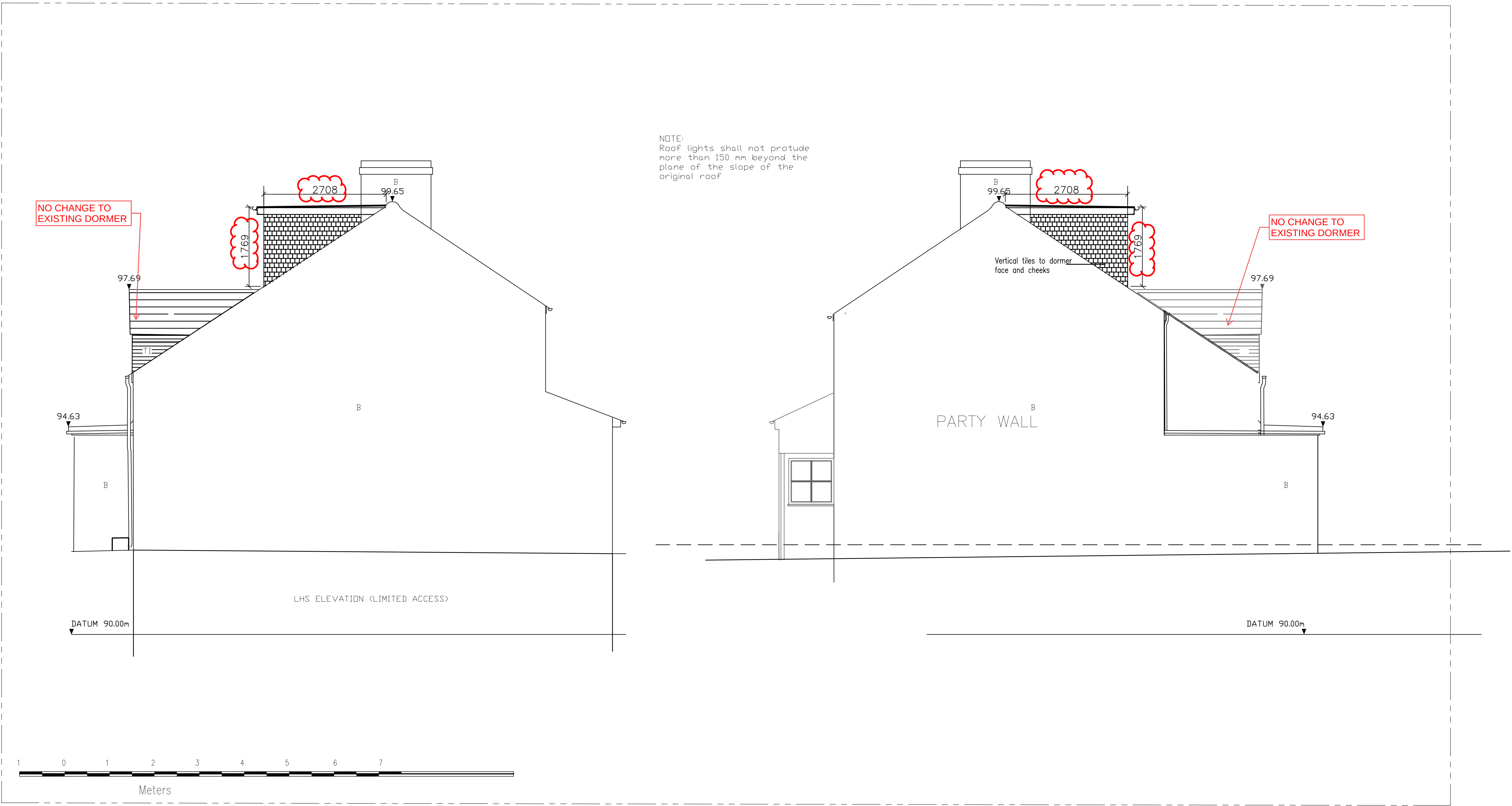
08 PRIOPOSED SIDE (EAST) ELEVATIONS
