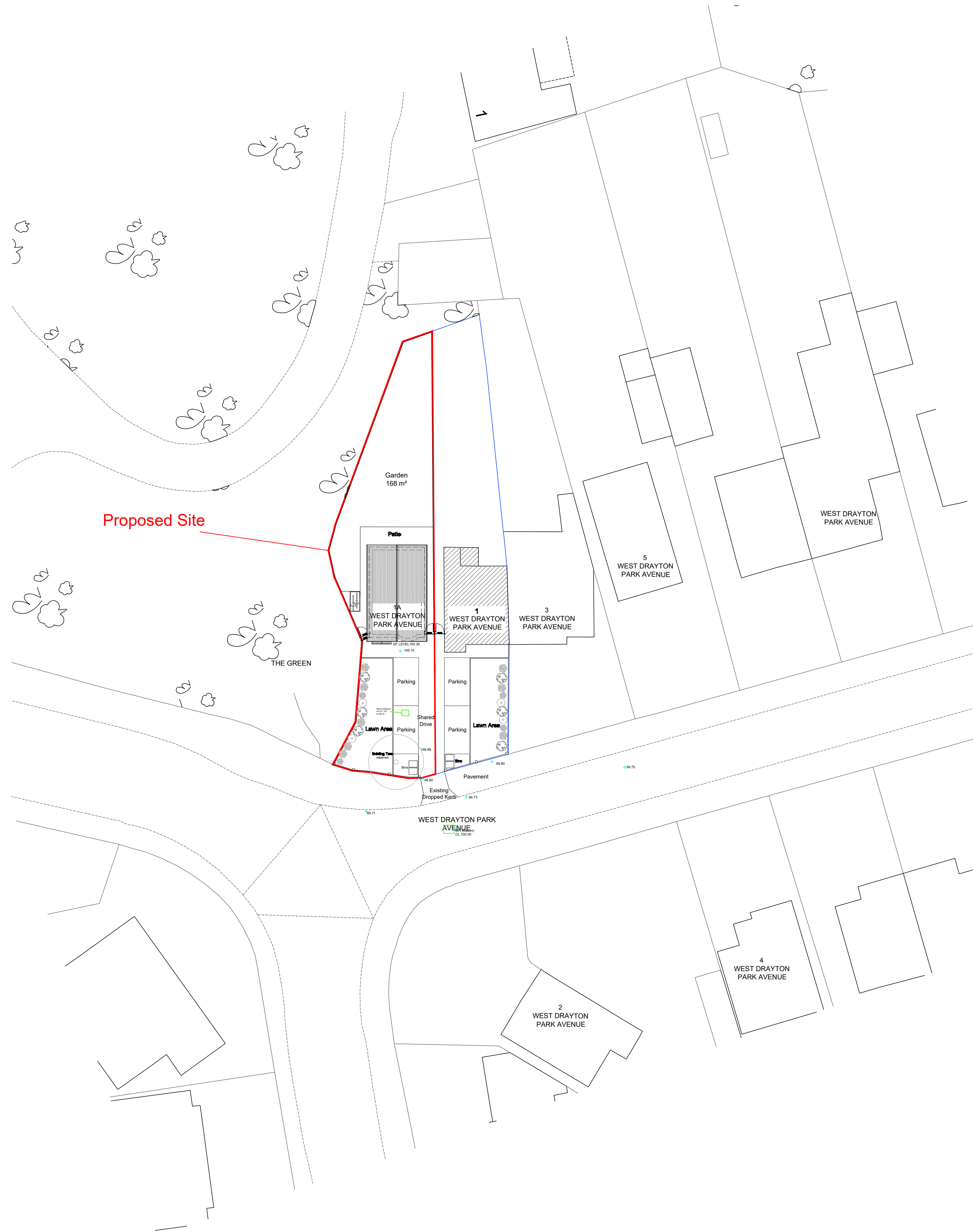
PROPOSED BLOCK PLAN SCALE 1:50
