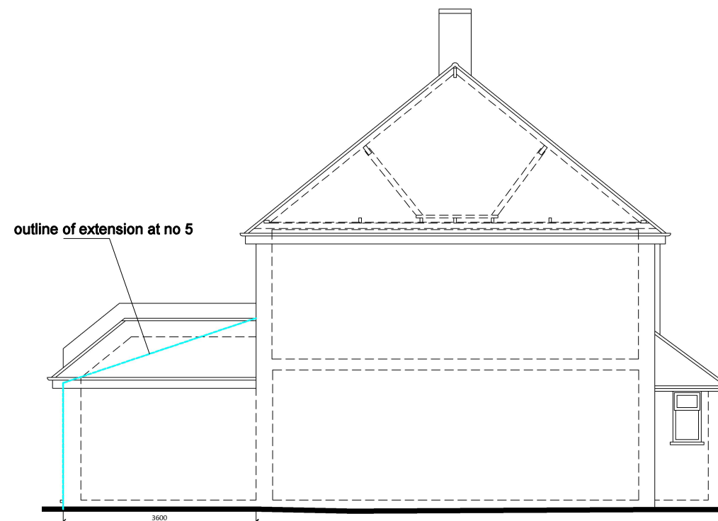
Proposed side elevation/section 1:100 (as seen from no 5)
