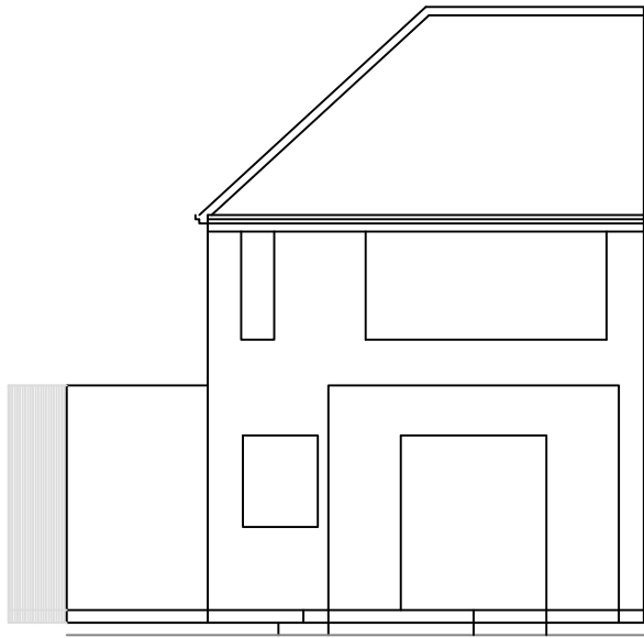
REAR ELEVATION
