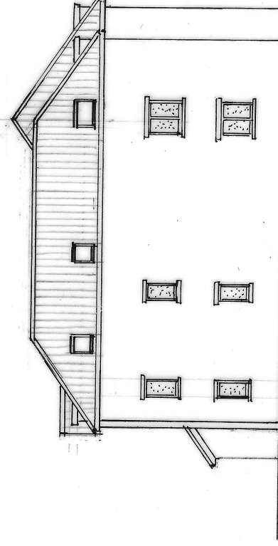
EAST ELEVATION
