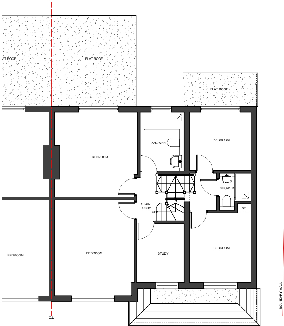
02- FIRST FLOOR PLAN
