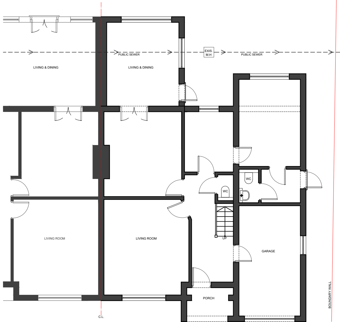
01- GROUND FLOOR PLAN
