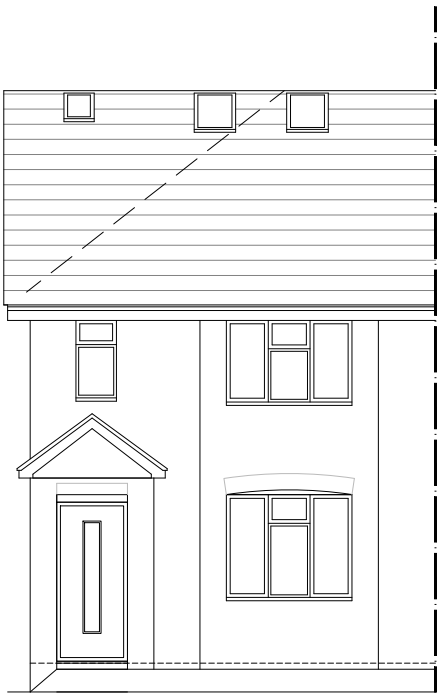
FRONT ELEVATION
