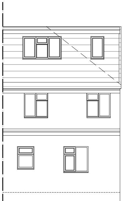
REAR ELEVATION
