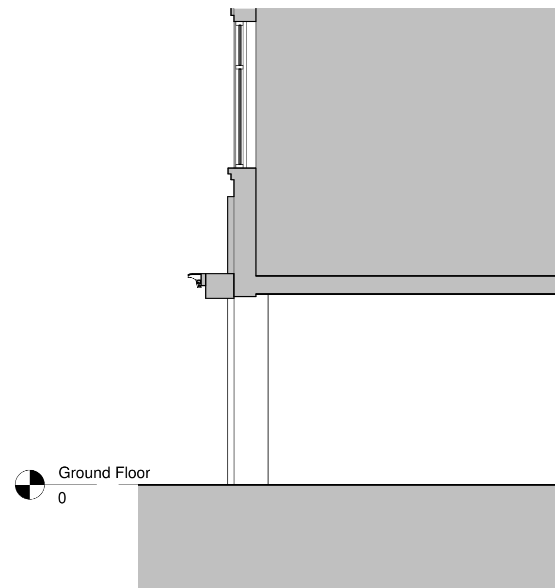
Section AA Closed Canopy 1 : 50
