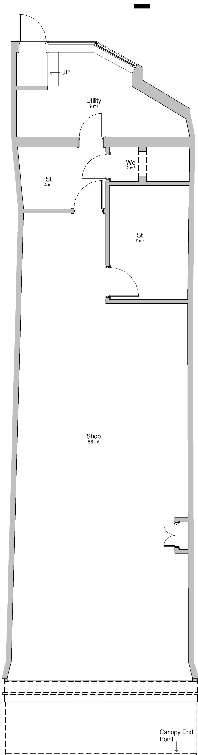
Ground Floor 1 : 50
