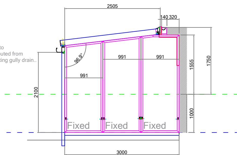
RHS View
