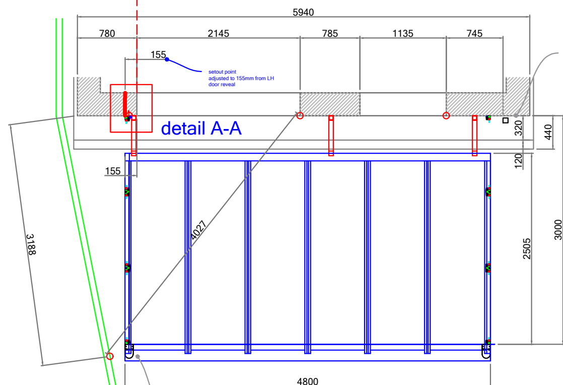
Plan View
