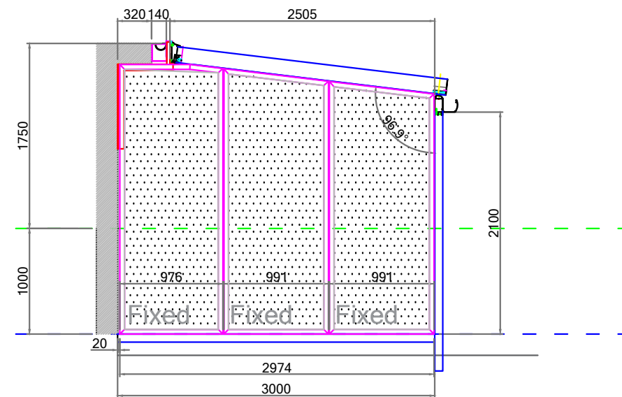
LHS View
