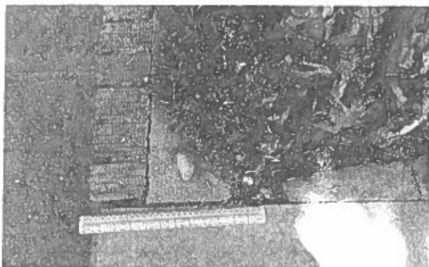
Figure 4 Retaining wall displaced by 20 mm.
