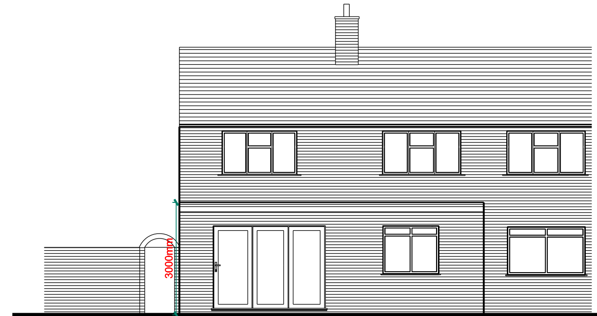
03 PREVIOUSLY APPROVED REAR ELEVATION APPLICATION REF : 17286/APP/2024/2774 SCALE 1:100
