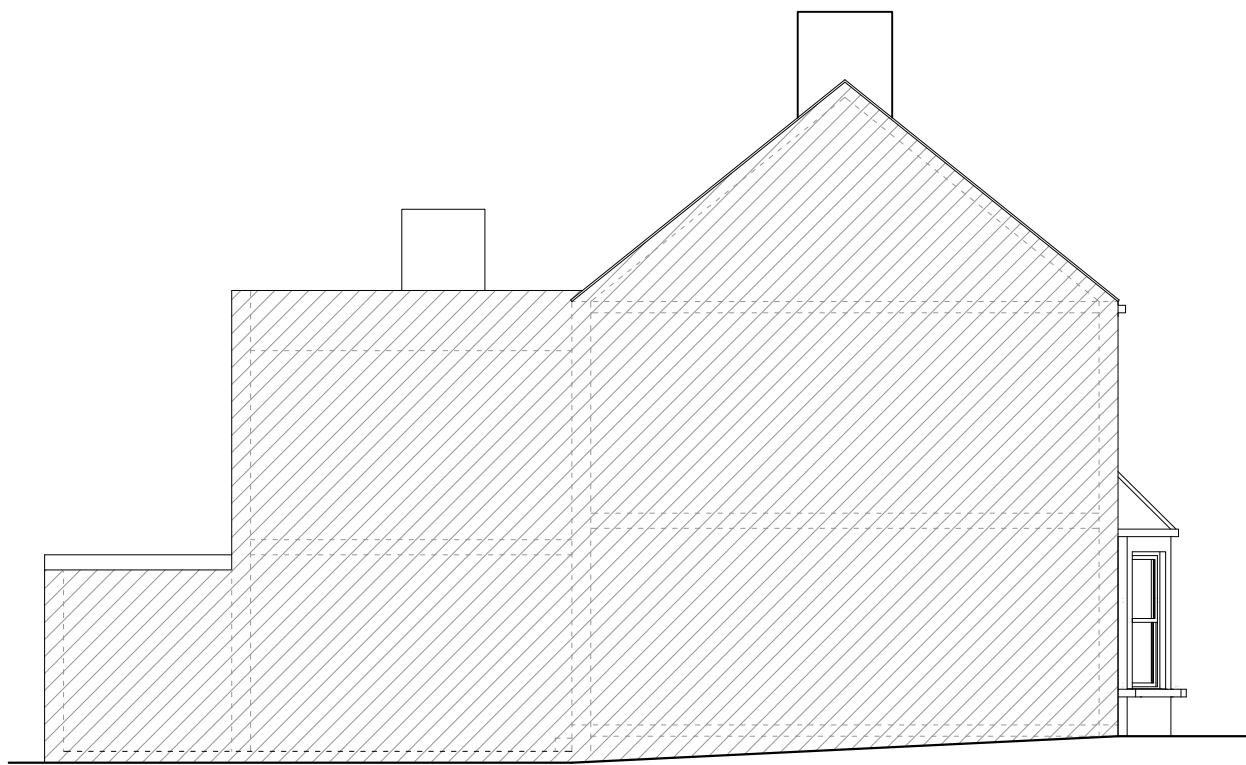
Proposed side elevation (A)
