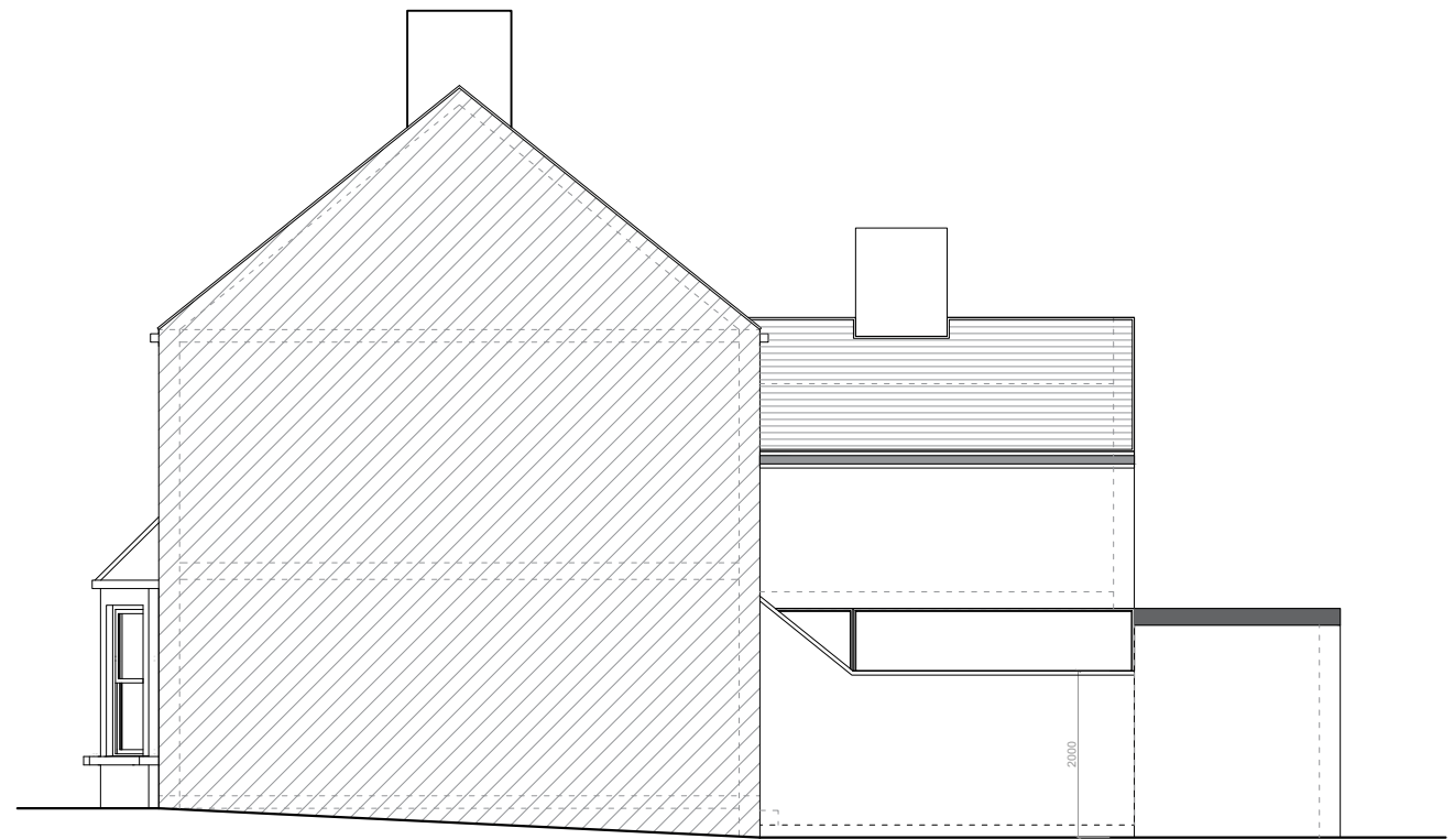
Proposed side elevation (B)
