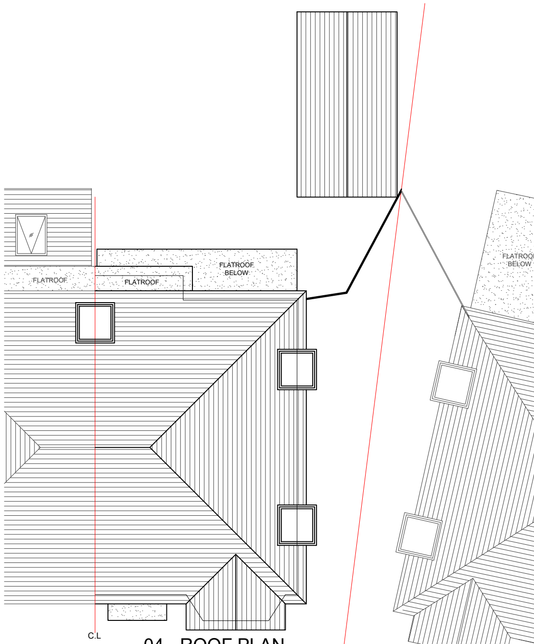
04 - ROOF PLAN
