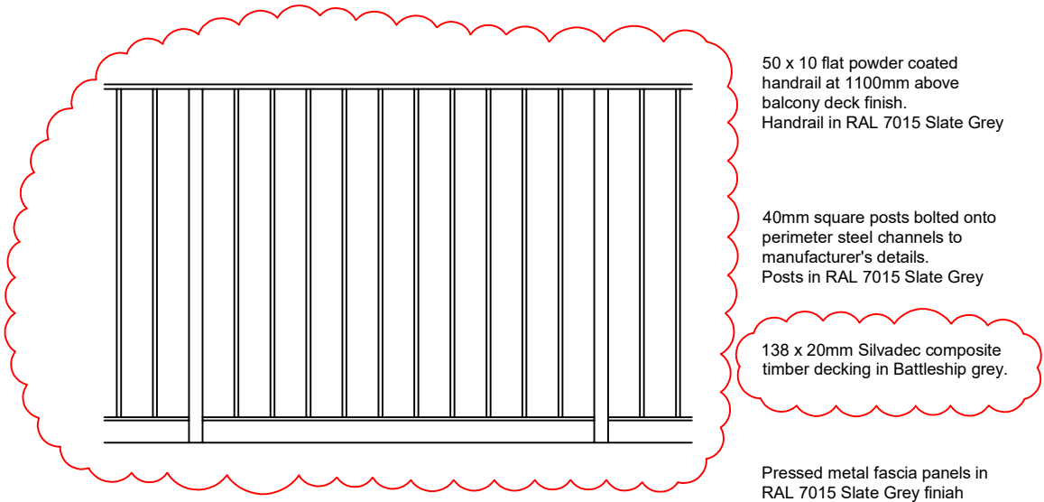
PART TYPICAL ELEVATION
