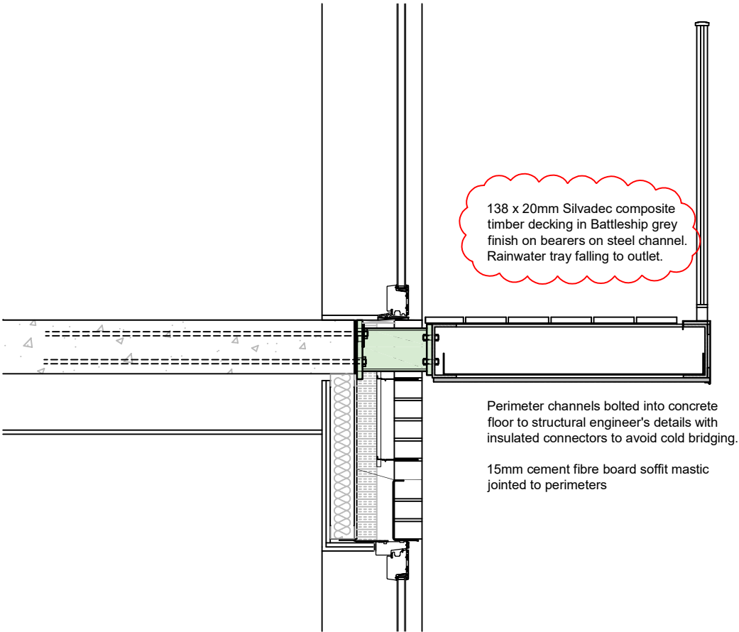
TYPICAL SECTION AT FLOOR INTERSECTION
