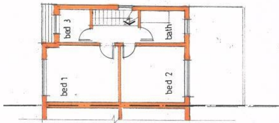
FIRST FLOOR
