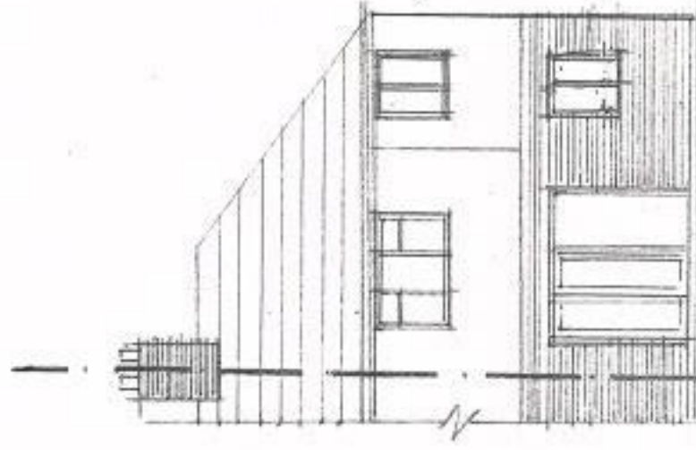
GARDEN ELEVATION
