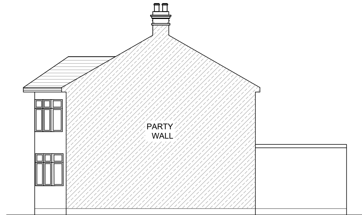
PROPOSED OTHER SIDE ELEVATION
