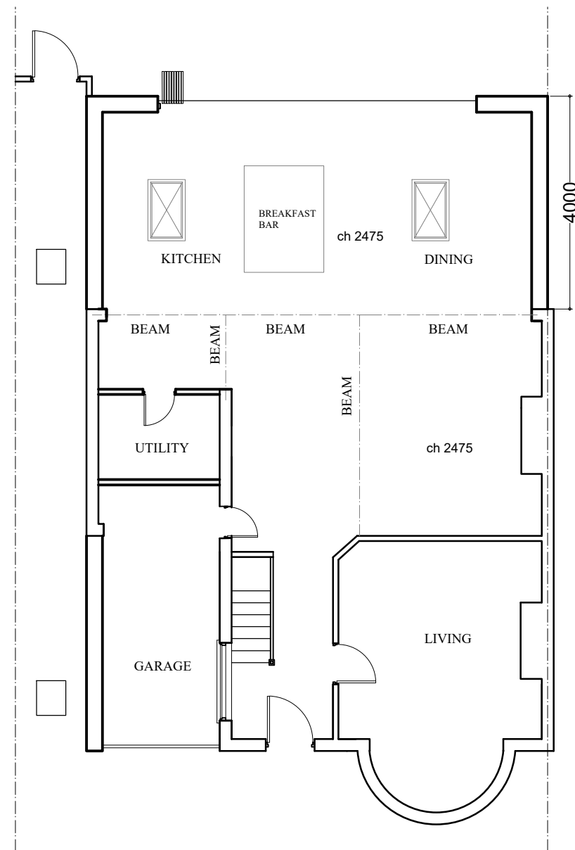
APPROVED GROUND FLOOR PLAN
