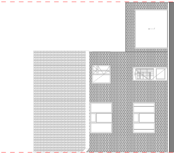
Rear Rear Elevation 1:100
