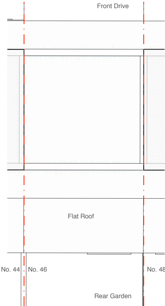
Existing Loft Plan
