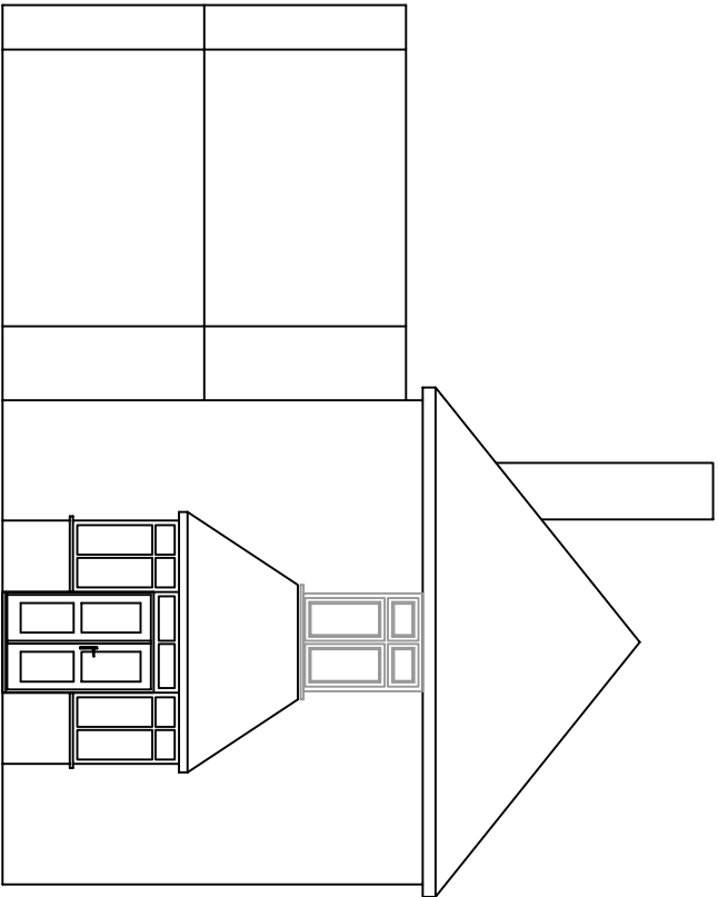
EXISTING LEFT ELEVATION
