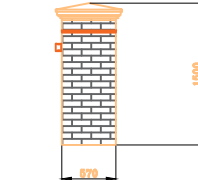
New Brick Pillars with root protection membrane
