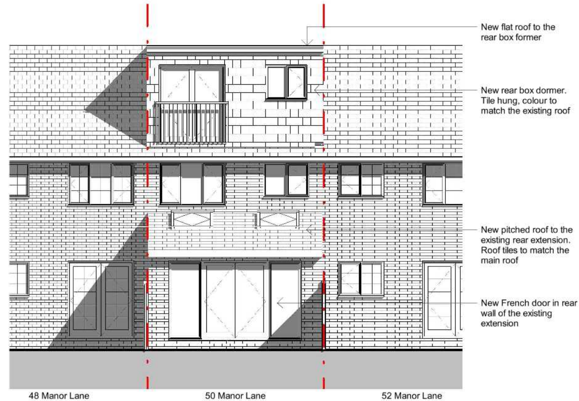
2 Rear Elevation as Proposed 1 : 100
