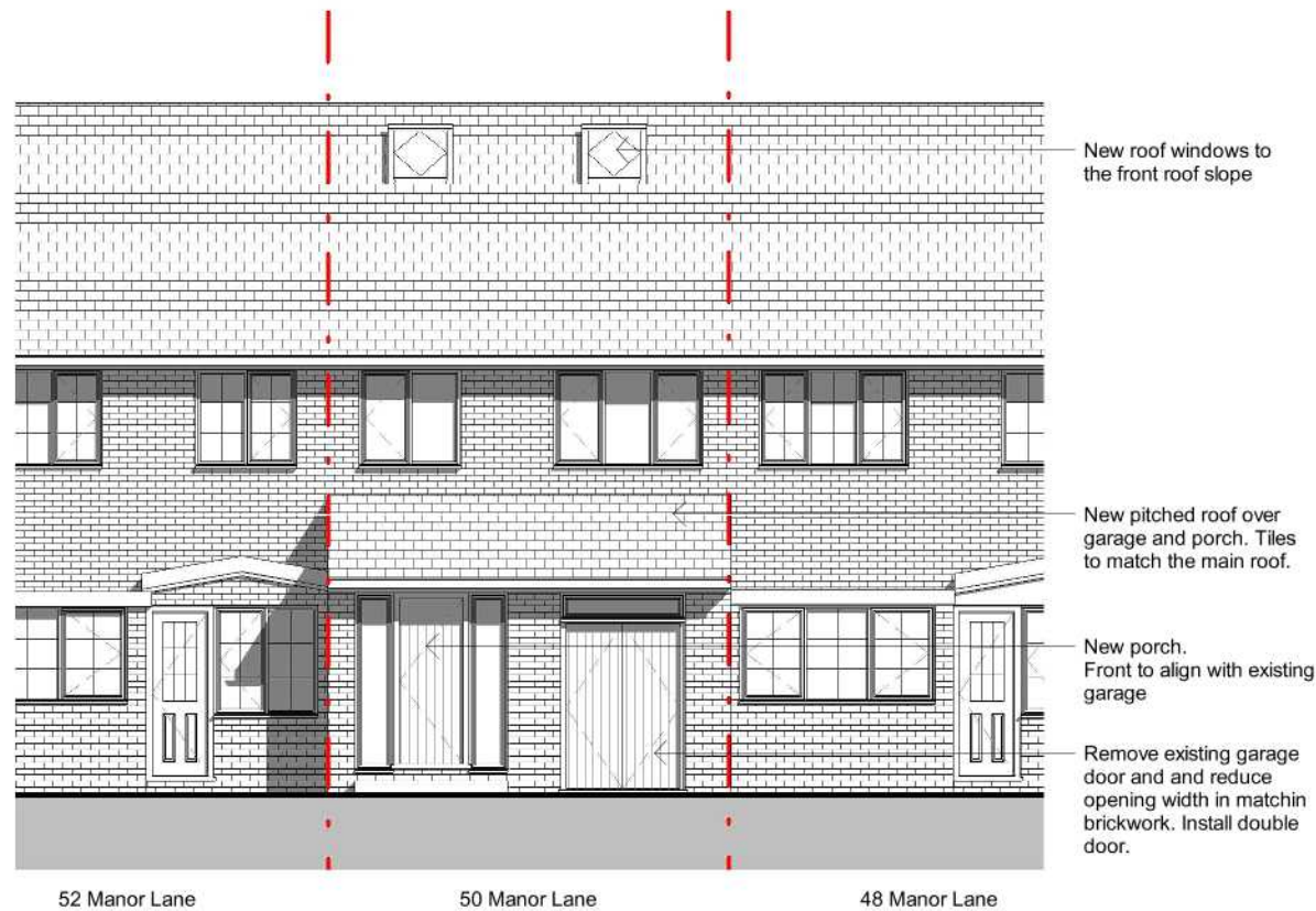
1 Front Elevation as Proposed 1 : 100
