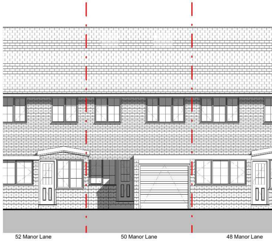
1 North (Front) Elevation as Existing 1 : 100
