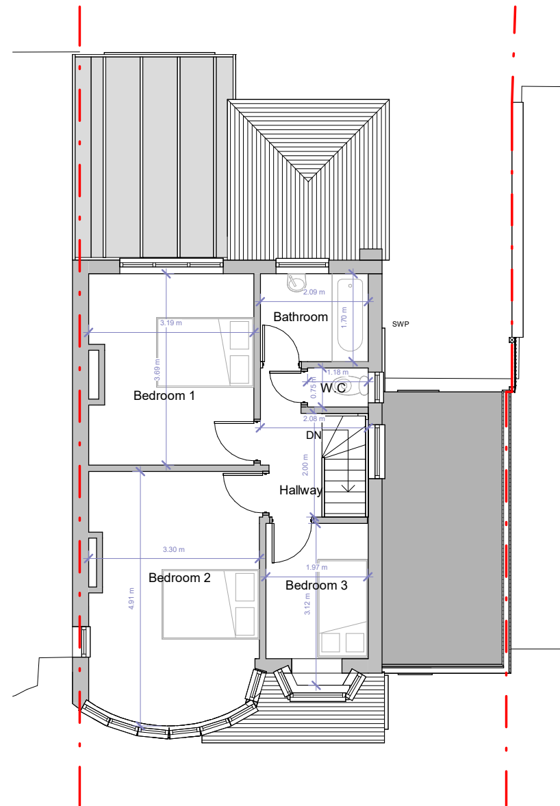
First Floor
