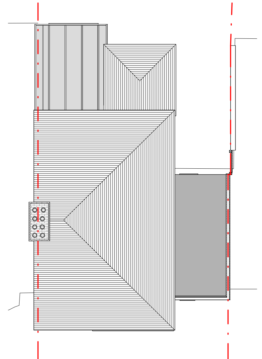
Roof Plan
