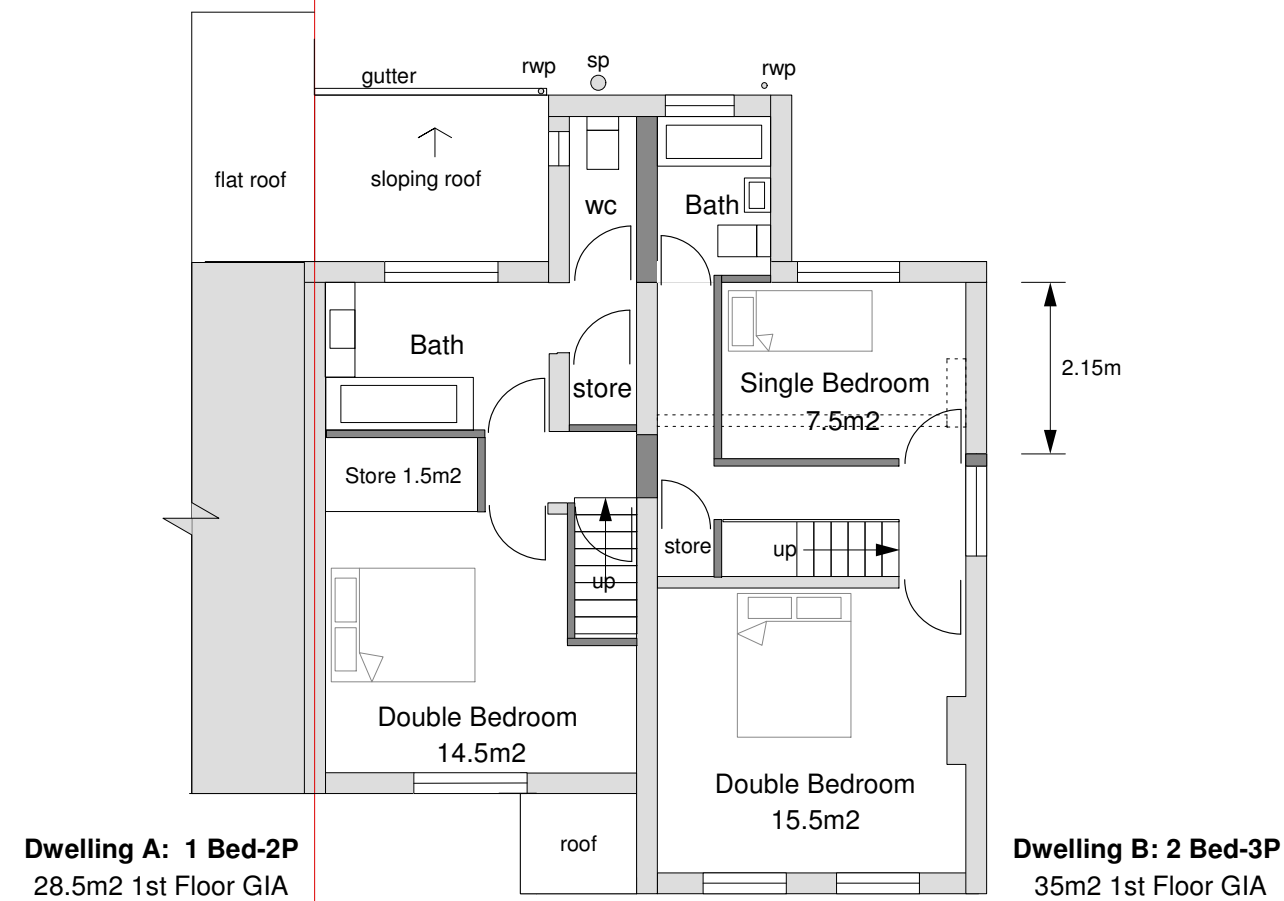
First Floor Proposed
