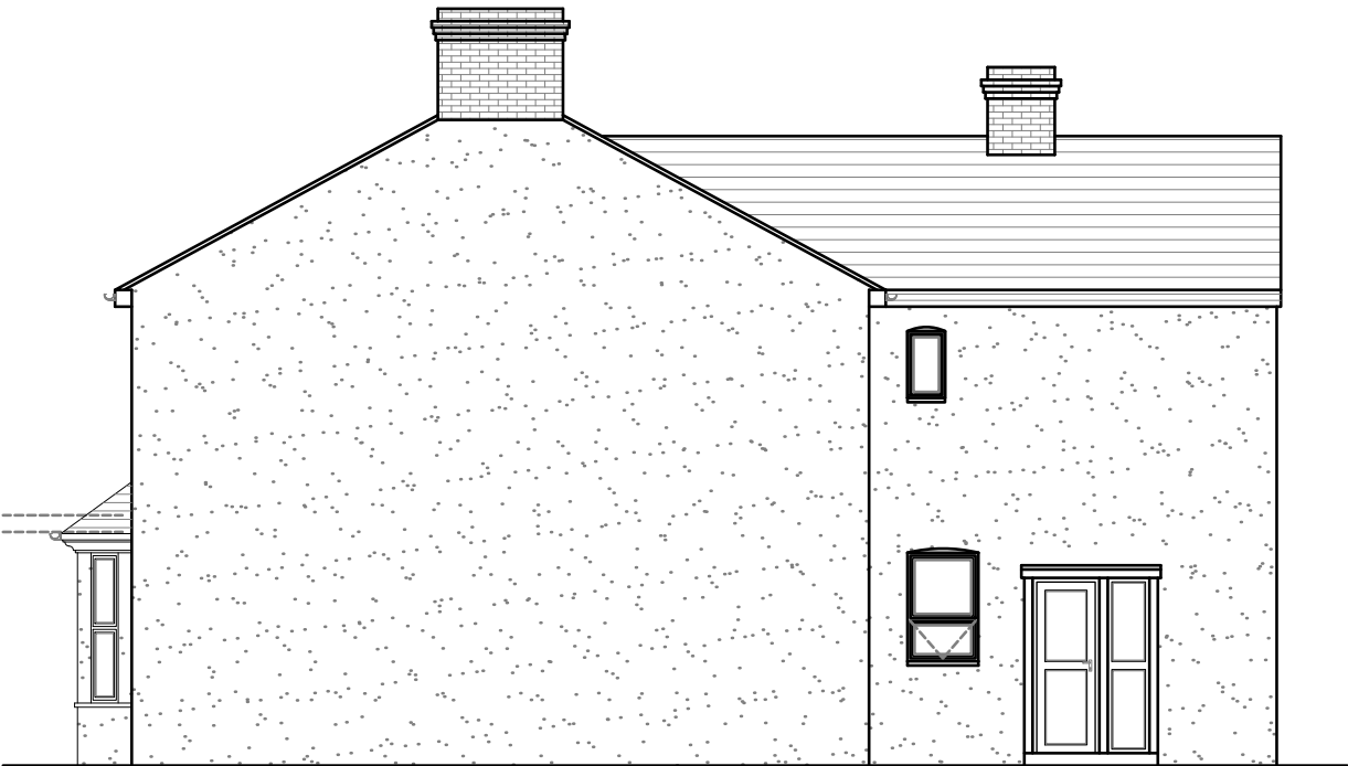
EXISTING EAST SIDE ELEVATION SCALE= 1:100
