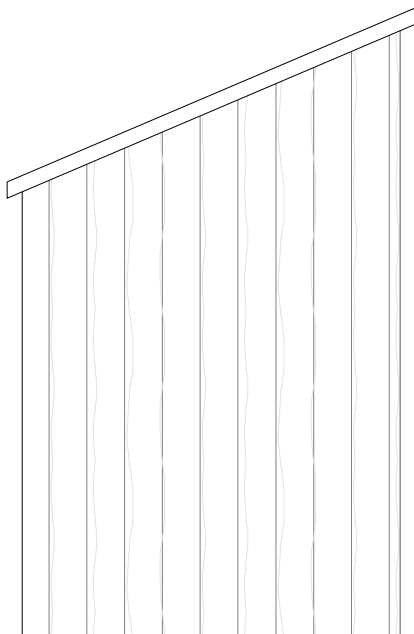
PROPOSED ELEVATION - SIDE I (SCALE 1:25)
