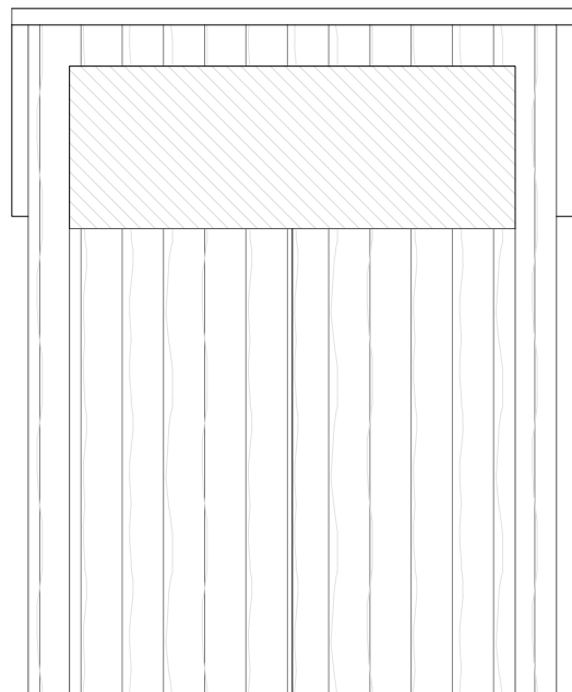
PROPOSED ELEVATION - FRONT (SCALE 1:25)
