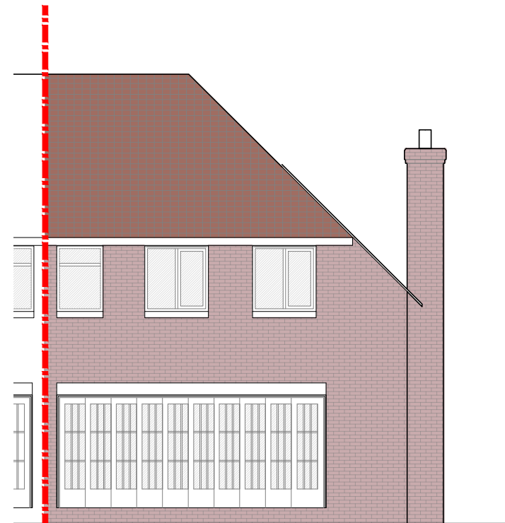
Existing Rear Elevation 1:100 Scale Bar 1:100
