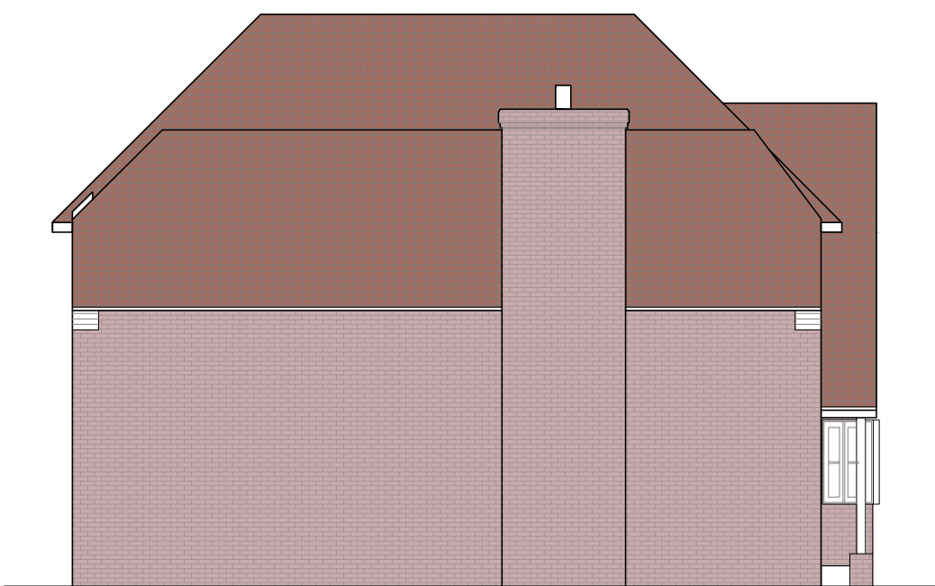
Existing East Elevation 1:100 Scale Bar 1:100
