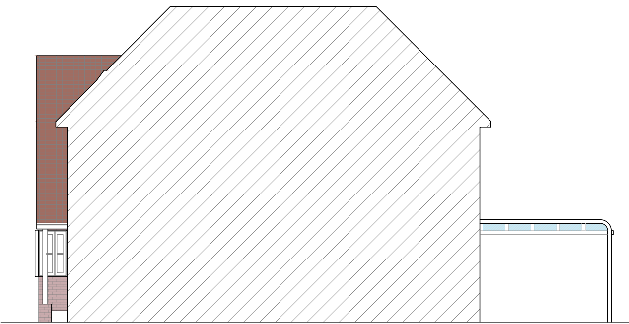
Proposed West Elevation 1:100 Scale Bar 1:100
