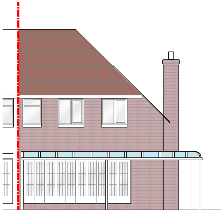
Proposed Rear Elevation 1:100 Scale Bar 1:100
