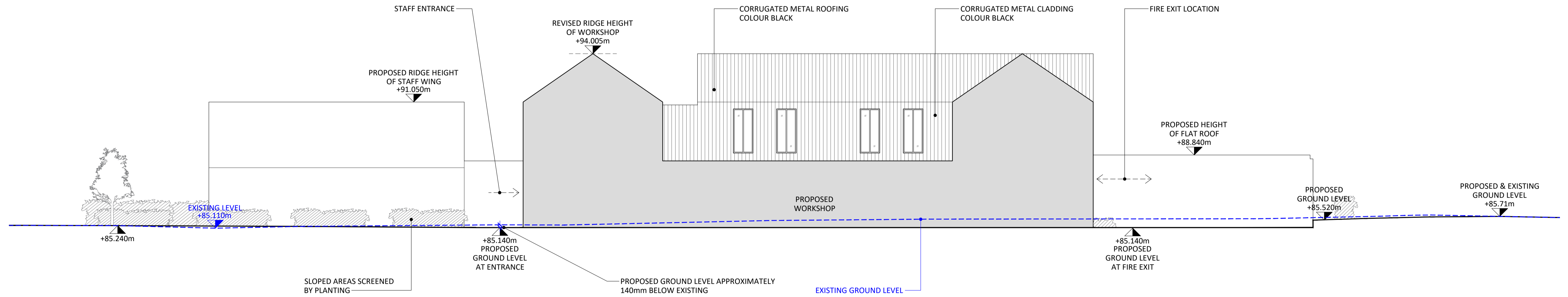
PROPOSED SITE SECTION F-F
