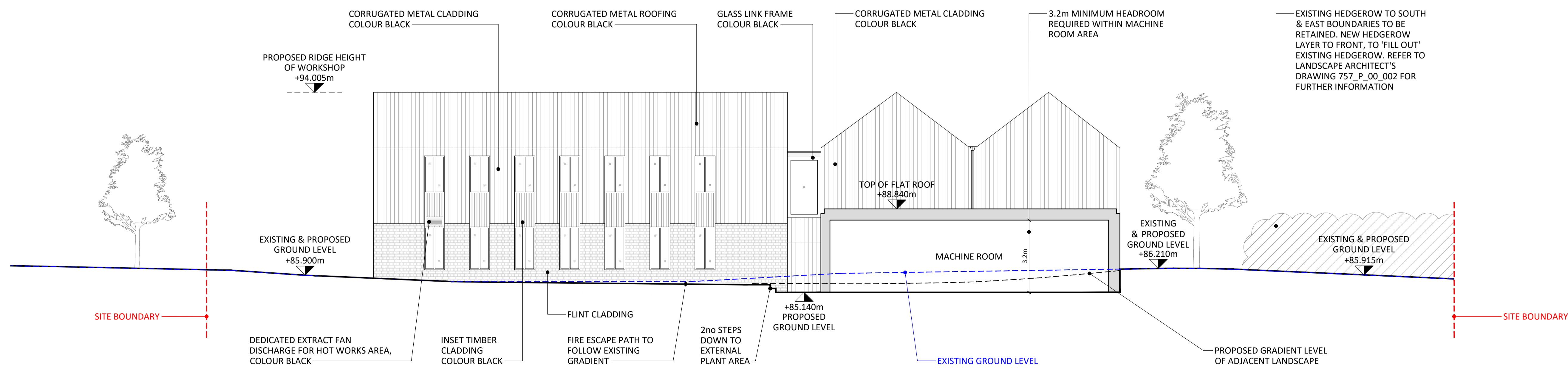
PROPOSED SECTION I-I
