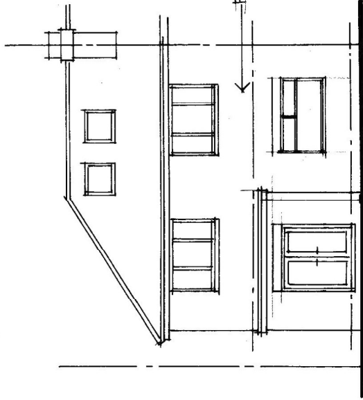
REAR - 1:100
