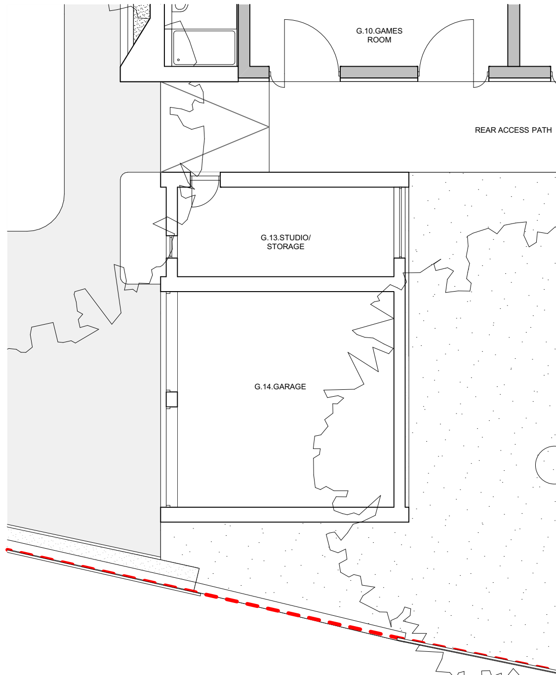
01 GARAGE GROUND FLOOR PLAN AS PROPOSED SCALE 1:100
