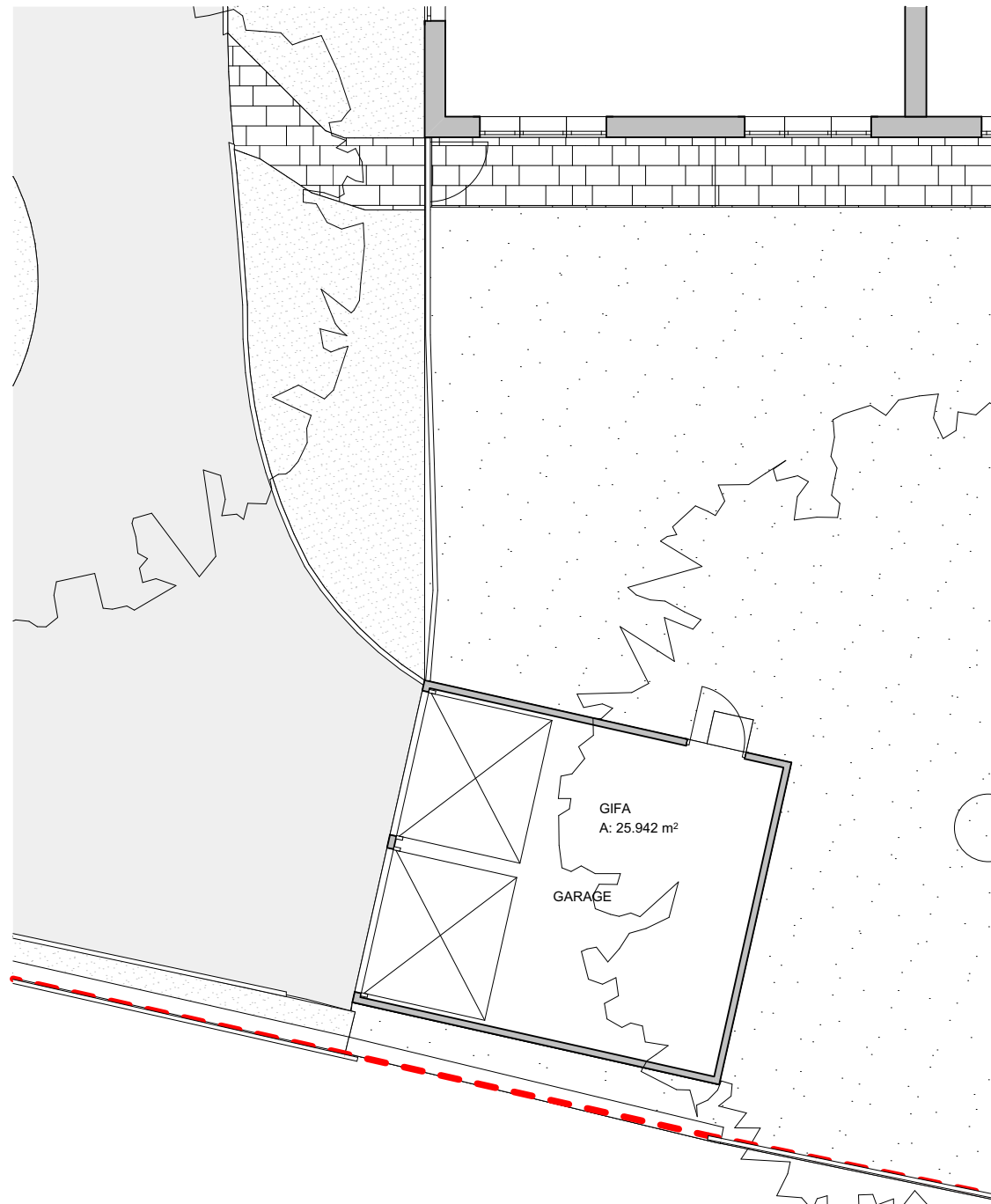
01 GARAGE GROUND FLOOR PLAN AS EXISTING 1104 SCALE 1:100
