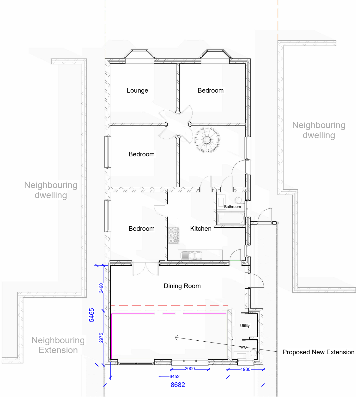
1 Proposed Ground Floor 1 : 100
