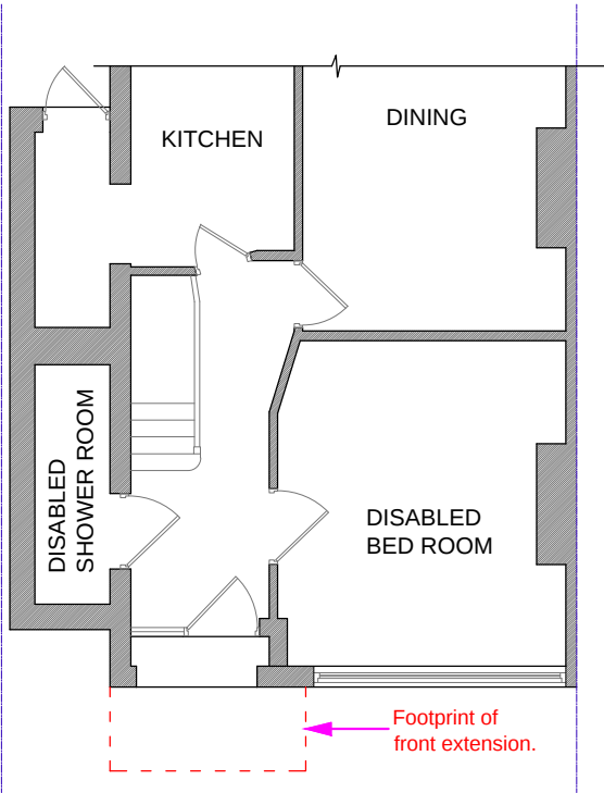
PRE-EXISTING GROUND FLOOR PLAN Scale 1:100
