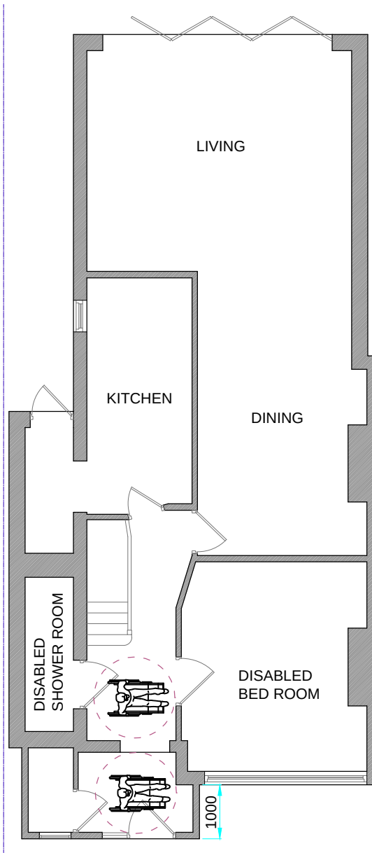
EXISTING/PROPOSED GROUND FLOOR PLAN Scale 1:100
