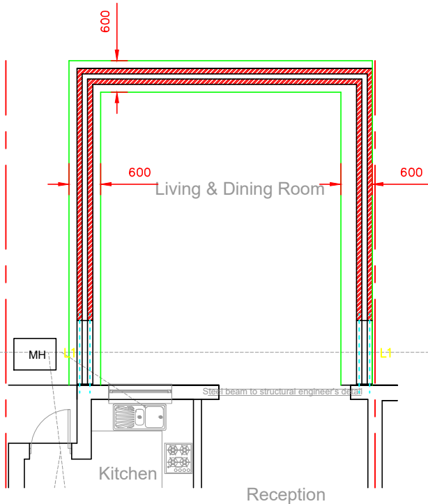
PROPOSED FOUNDATION GROUND FLOOR PLAN SCALE:-1:100
