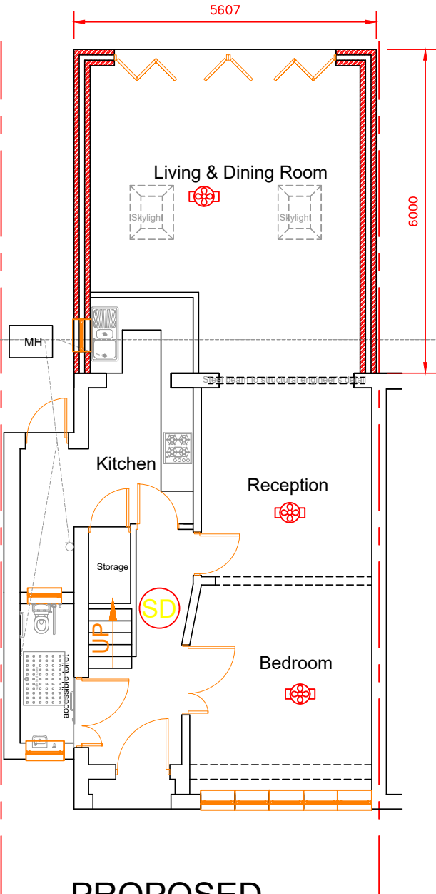
PROPOSED GROUND FLOOR PLAN SCALE:-1:100 WITH EXTERNAL BRICK FINISH AND AN OBSCURE WINDOW TO THE FLANK WALL
